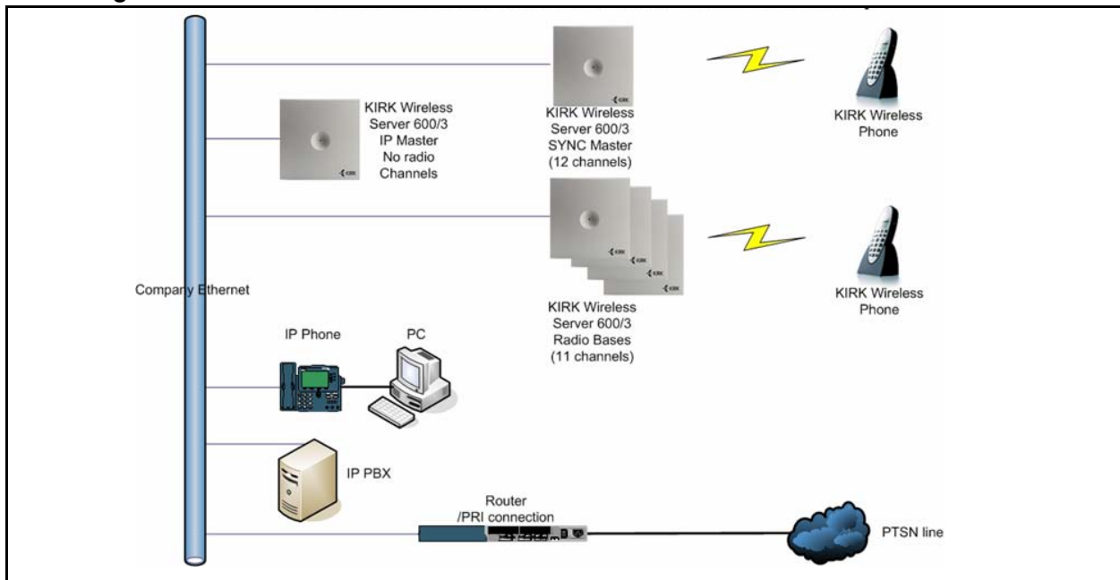
Figure 42 KWS600v3 Multi-cell installation
